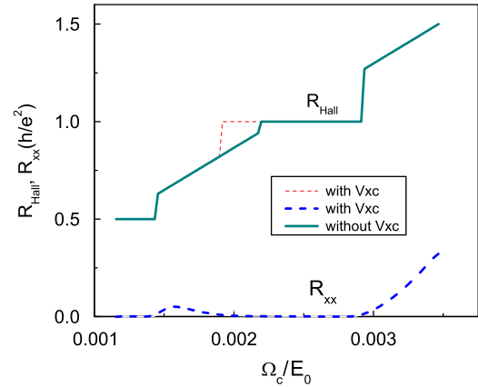
Fig. 4. Calculated Hall and longitudinal resistances versus scaled magnetic field \hbar\omega_c/E_0 , ignoring V_{xc} (solid line) and including V_{xc} (dashed line). Sample width of 2d = 3 \mu\text{m} and for a magnetic field of B = 7.1 T, at default temperature.
