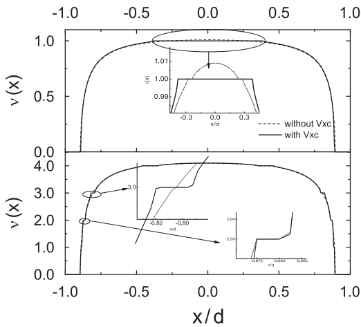
Fig. 3. Electronic ground state filling factors, neglecting V_{xc} (dashed line) and including V_{xc} (solid line) calculated for a sample width of 2d = 3 \mu\text{m} , at temperature T = 0.05 K and for magnetic fields: (a) B = 1.8 T, (b) B = 7.1 T.
