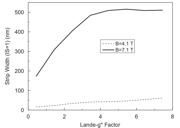
Fig. 1. The width of the first incompressible strip ( \nu = 1 ) without the exchange and correlation as a function of bulk Lande- g^* factor at T = 0.05 K, in a sample of width 3 \mu\text{m} , and for magnetic fields B = 4.1 T (dotted line) B = 7.1 T (solid line).
