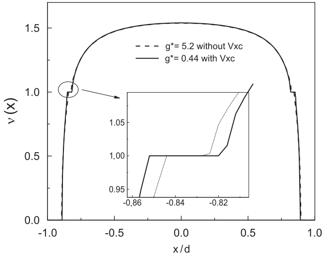
Fig. 2. The spatial variation of filling factor obtained from experimental effective Landé- g^* factor [10] ignoring V_{xc} (dashed line) and bulk Landé- g^* factor including V_{xc} (solid line). Calculations are performed at default temperature and at B = 4.7 T.
