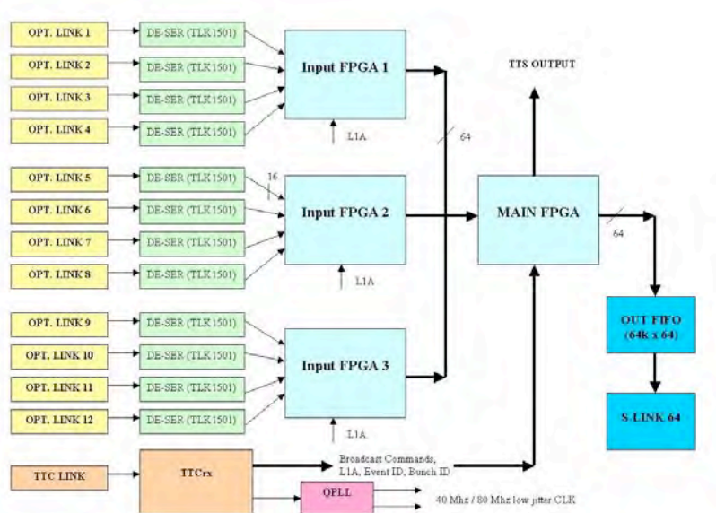
Figure 7.18: Scheme of the DDU architecture.
