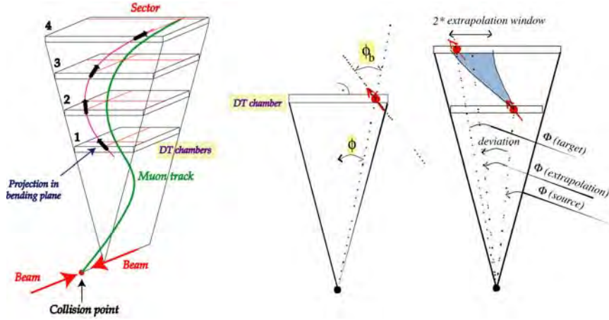
Figure 8.6: Track Finder extrapolation scheme.
