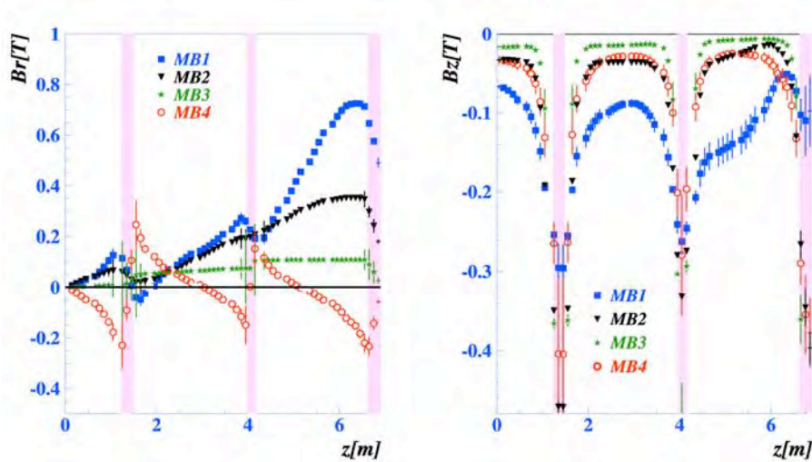
Figure 7.32: Radial ( B_r ) and longitudinal ( B_z ) components of the CMS magnetic field in the regions where the barrel chambers are placed as a function of the position along the beam direction (the centre of the detector is at z=0 ). Vertical bands indicate the separation between chamber wheels (in these particular regions B_z becomes significant). The biggest B_r values (0.7–0.8 T) occur in the MB1 region near the endcaps.
