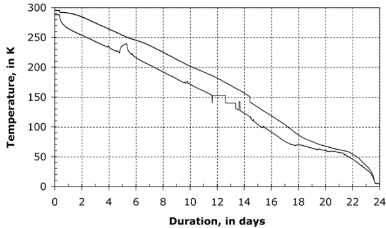
Figure 2.9: Graph of the coil minimum and maximum temperatures during the cool-down from room temperature to 4.5 K.
