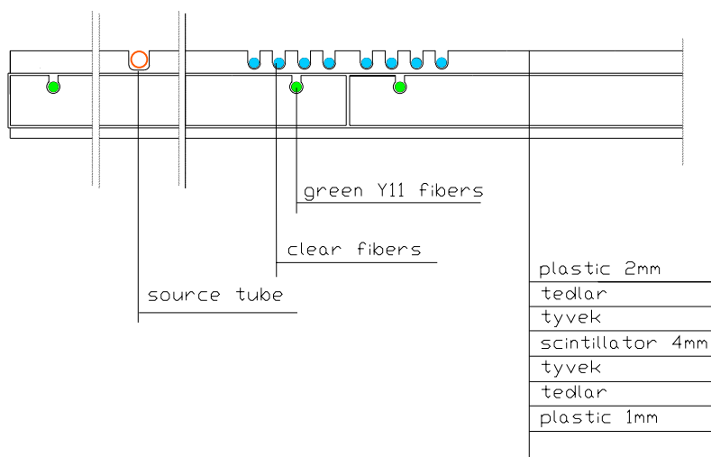
Figure 5.6: Cross-sectional view of a scintillator tray.
