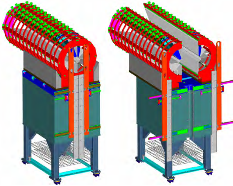
Figure 6.2: CASTOR calorimeter and support.
