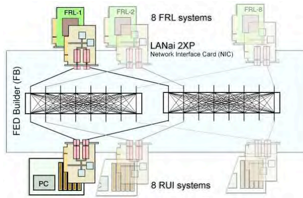
Figure 9.9: 8×8 FED builder with a two-rail network.
