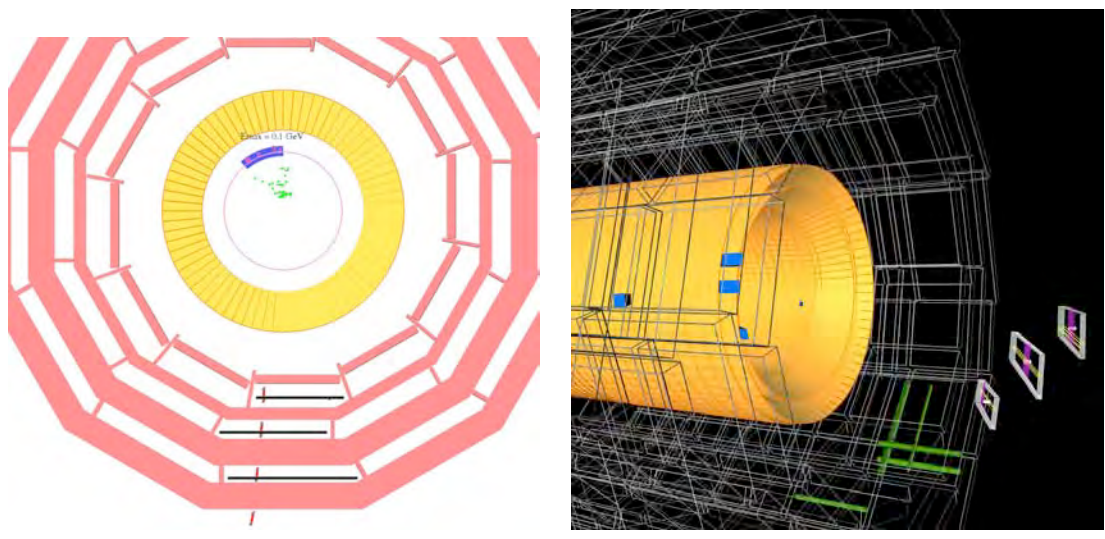
Figure 7.44: Event displays from the MTCC. Left panel: muon reconstructed in a DT sector in conjunction with Tracker activity. Right panel: muon track passing through both DT and CSC chambers.
