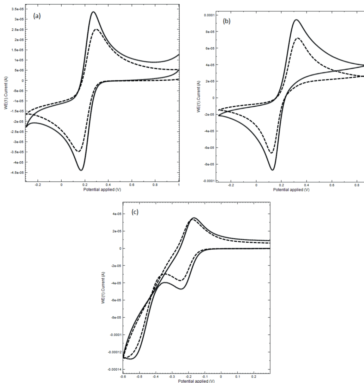
Figure 4. Cyclic voltammograms for a) 1 \times 10^{-3} M \text{K}_3\text{Fe}(\text{CN})_6 , b) 1 \times 10^{-3} M catechol, c) 1 \times 10^{-3} \text{Ru}(\text{NH}_3)_6^{3+} . Straight line: BCPE (Biochar/graphite/oil ratio of 2/68/30 (w/w) %), dashed line: CPE (graphite/oil 70/30 (w/w) %).
