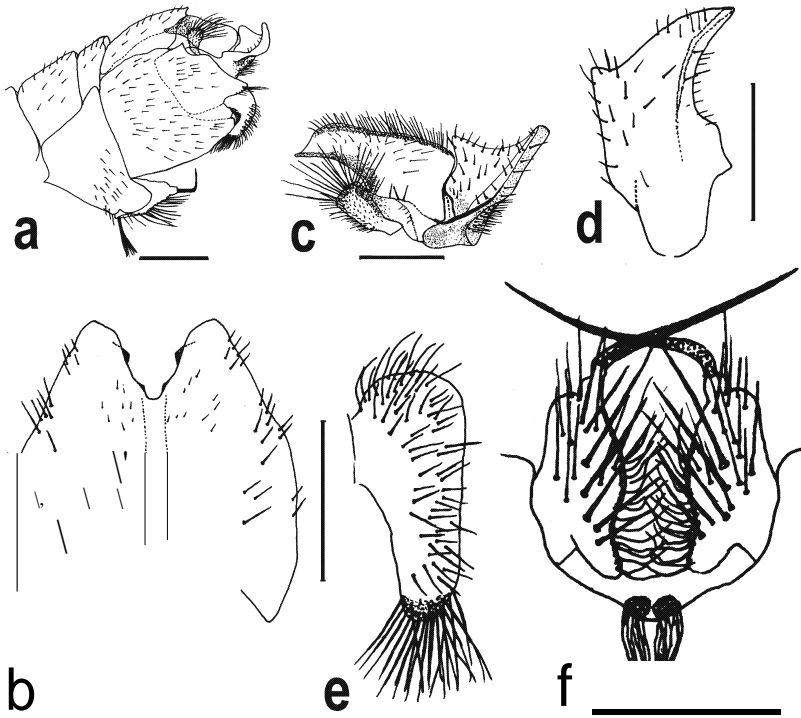
Fig. 1. Tipula (Lunatipula) murati sp. n. - a. Hypopygium, lateral view. - c. Left inner and outer gonostyles, outside view. - d. Left inner gonostyle, from behind. - b. Tergite 9, dorsal view. - f. Hind margin of stemite 8 and the bristle bearing lobes, hind view. - e. Appendage of stemite 9, lateral view. Scale bars 1.0 mm (a, b, f) and 0.5 mm (c, d, e).
