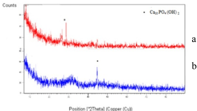
Figure 2. XRD patterns of 45S5-SrR a) before SBF b) on 28th day in SBF
