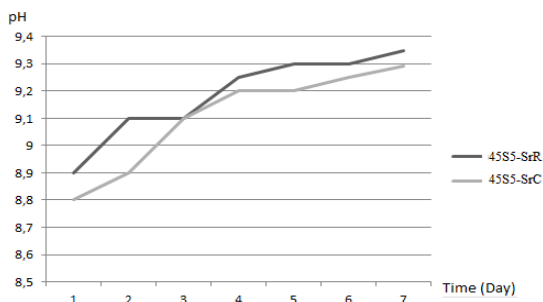
Figure 5. The pH variation of TRIS solution with soaking time for 45S5-SrR and 45S5-SrC sample
