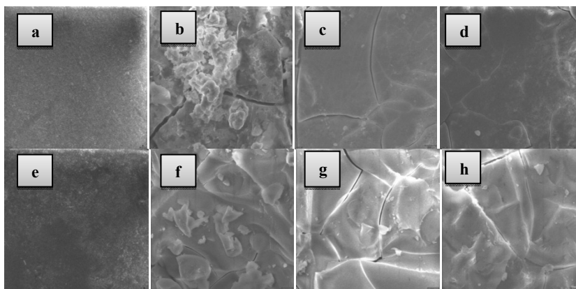
Figure 1. SEM micrographs showing the morphology of the 45S5-SrR sample a) before SBF, b) on 7th day in SBF, c) on 14th day in SBF, d) on 21th day in SBF and 45S5-SrC sample e) before SBF, f) on 7th day in SBF, g) on 14th day in SBF, h) on 21th day in SBF
