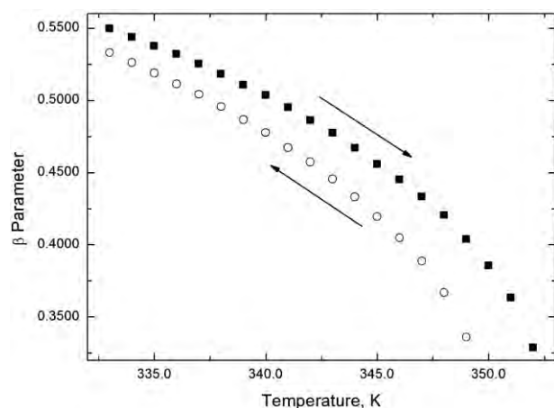
Fig. 14. Temperature dependences of the \beta parameter. ■ – values for heating process; ○ – values for cooling process.
