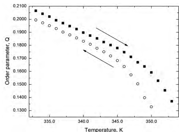
Fig. 12. Temperature dependences of the order parameter Q . \blacksquare – Q = Q(T) dependence for heating process; \circ – Q = Q(T) dependence for cooling process.
