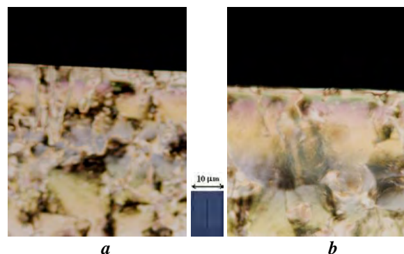
Fig. 4. Biphasic regions of the N-I (a) and I-N (b) phase transitions. Crossed polarizers; Magnification \times 100 .
