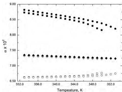
Fig. 8. Temperature dependences of the polarizabilities. ● – \alpha_e values for heating process; ○ – \alpha_o values for heating process; ■ – \alpha_e values for cooling process; □ – \alpha_o values for cooling process; ◆ – \alpha_{ave} values for heating process; ◇ – \alpha_{ave} values for cooling process.
