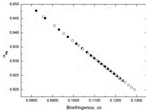
Fig. 10. The \alpha_{eg} = \alpha_{eg}(\Delta n) dependences for the heating ( \circ ) and cooling ( \blacksquare ) processes.
