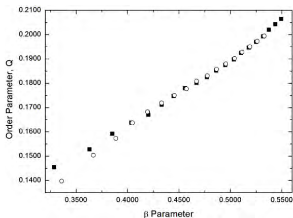
Fig. 13. The Q = Q(\beta) dependences for the heating (■) and cooling (○) processes.
