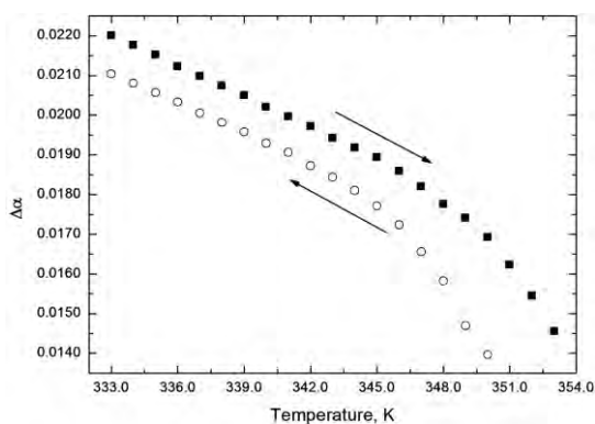
Fig. 11. Temperature dependences of the \Delta\alpha . \blacksquare – values for heating process; \circ – values for cooling process.
