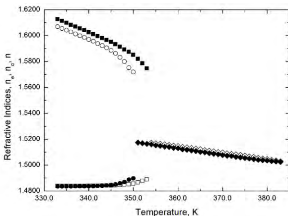
Fig. 6. Temperature dependences of the refractive indices. ■ – n_e values for heating process; □ – n_o values for heating process; ○ – n_e values for cooling process; ● – n_o values for cooling process; ◇ – n values for heating process; ◆ – n values for cooling process.
