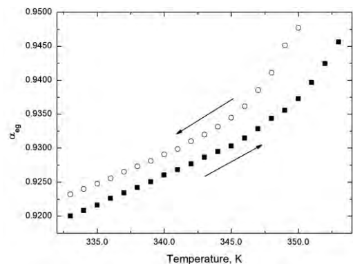
Fig. 9. Temperature dependences of the \alpha_{eg} . ■ – values for heating process; ○ – values for cooling process.
