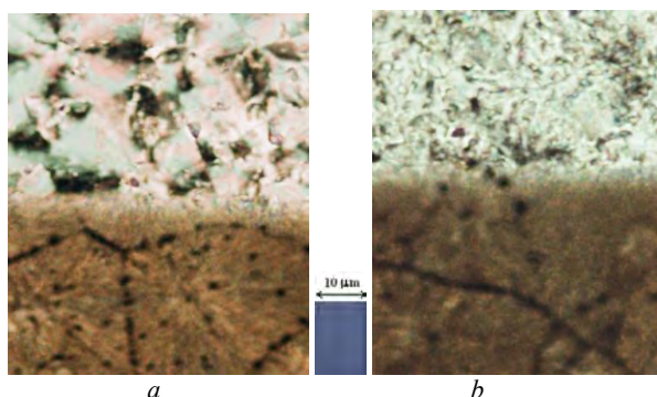
Fig. 3. Biphasic regions of the Cr-N (a) and N-Cr (b) phase transitions. Crossed polarizers; Magnification \times 100 .
