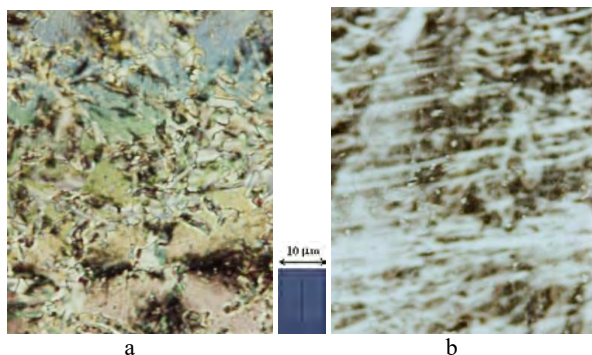
Fig. 1. Typical textures of nematic mesophase in BPHB. Crossed polarizers; Magnification \times 100 ; – Temperature 340.0 K; b – temperature 343.3 K.
