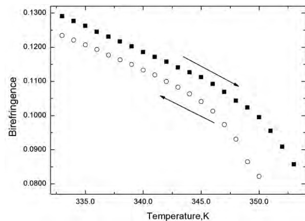
Fig. 7. Temperature dependences of the birefringence. ■ – \Delta n values for heating process; ○ – \Delta n values for cooling process.
