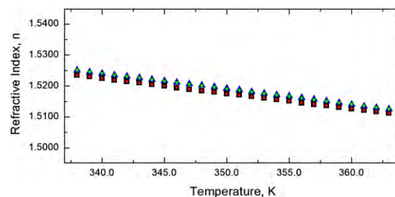
Fig. 5. Temperature dependences of the refractive index n . \blacktriangle – experimental values for heating process; \blacktriangledown – fitting values for heating process; \blacksquare – experimental values for cooling process; \bullet – fitting values for cooling process.
