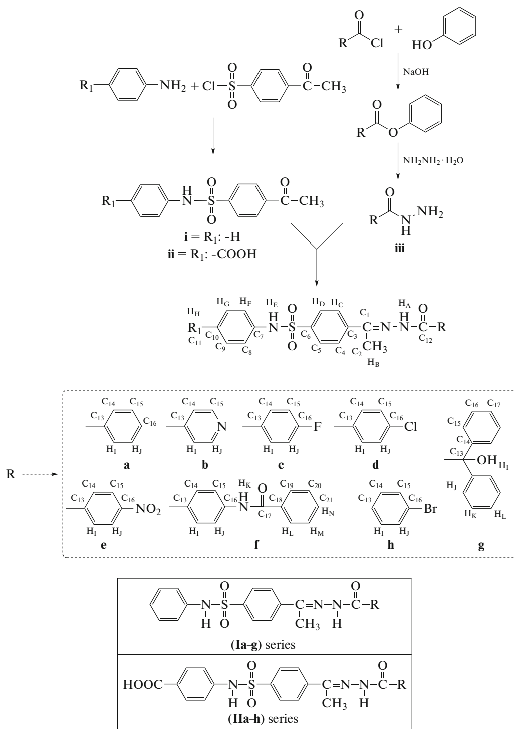
Scheme 1. Synthetic pathway of substituted hydrazide-hydrazones ( Ia–g ), ( IIa–h ).
